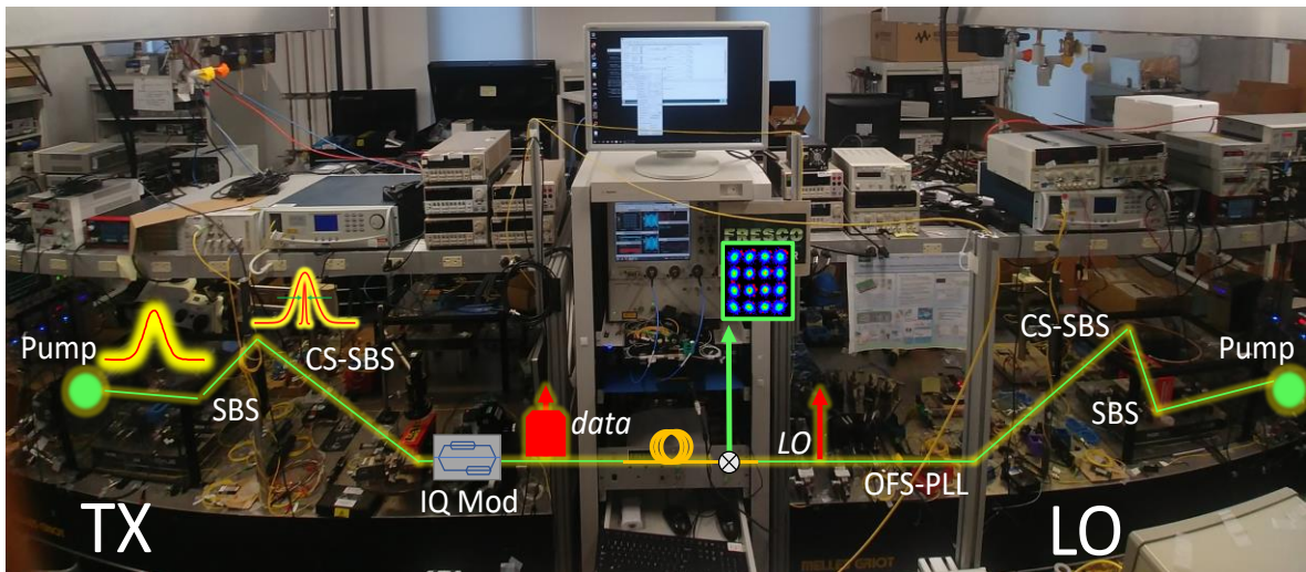
Figure 6.13. Laboratory setup of the FREquency Stabilized Coherent Optical (FRESCO) link. Two cavity-stabilized SBS lasers (SBS) serve as the transmit (TX) and local oscillators. Carrier phase recovery is realized using the optical-frequency stabilized phase locked loop (OFS-PLL). Coherent data and constellation recovery is performed using a commercial optical modulation analyzer (OMA).
