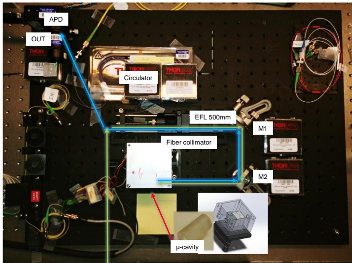
Figure 4.7. Tabletop setup of fiber collimator to free space coupling of the laser mode to the fundamental cavity mode of the Fabry-Perot resonator. A lens with 500 mm effective focal length and two turning kinematic-mounted mirrors enabled optical alignment.
