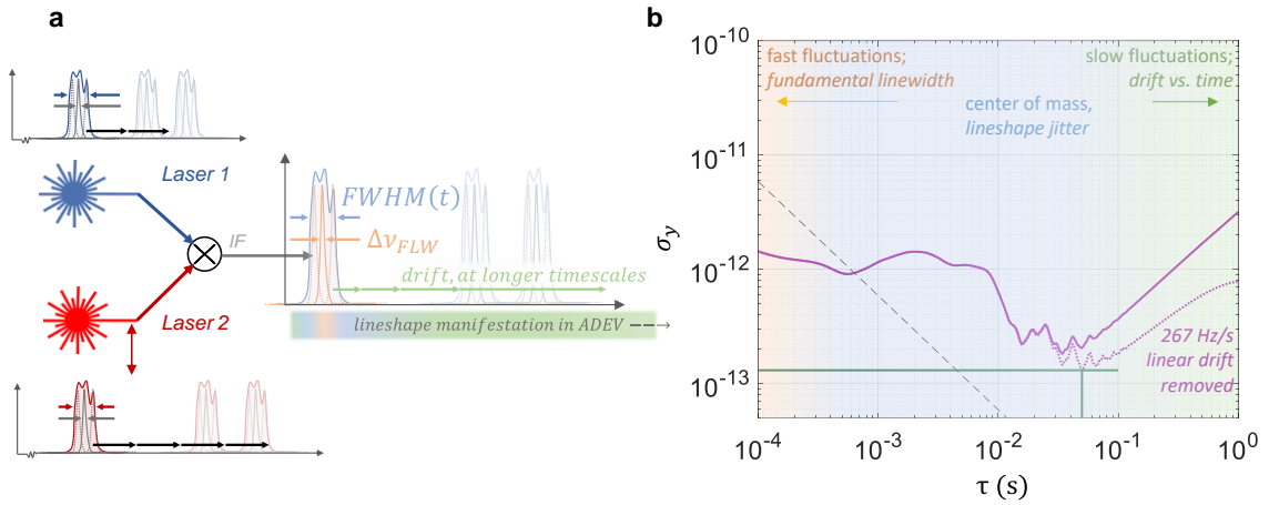
Figure 3.11. (a) Two lasers are heterodyned to generate an intermediate frequency (IF) signal to be measured by electrical frequency discriminator. The IF signal inherits the combined noise and stability of each of the independent lasers. (b) Sample ADEV plot (purple) with labeled regions governed by fast, center of mass, and slow fluctuations in the measured fractional frequency instability. A linear drift of 267 Hz/s is subtracted (purple, dotted).
