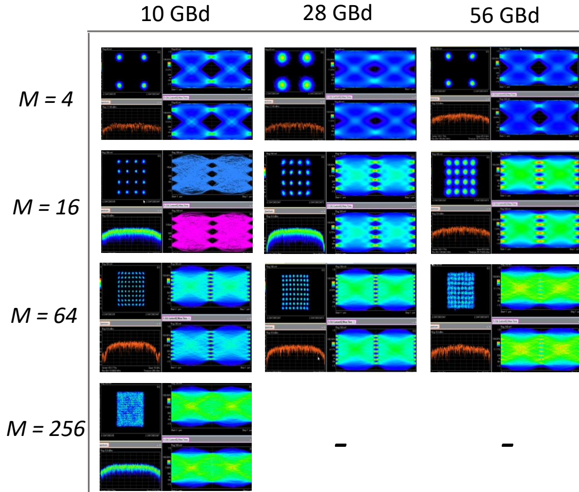
Figure 6.16. FRESCO constellations and eye diagrams for symbol rates of 10, 28, and 56 GBd and modulation orders M = 4 -, 16-, 64-, and 256-QAM. **For the 10- and 28 GBd 4-QAM tiles, the receiver did not include an optical preamplifier EDFA resulting in the higher SNR constellations in comparison to 56GBd 4-QAM. Transmission of 256-QAM at data rates of 28 and 56 GBd was not achieved in these demonstrations
