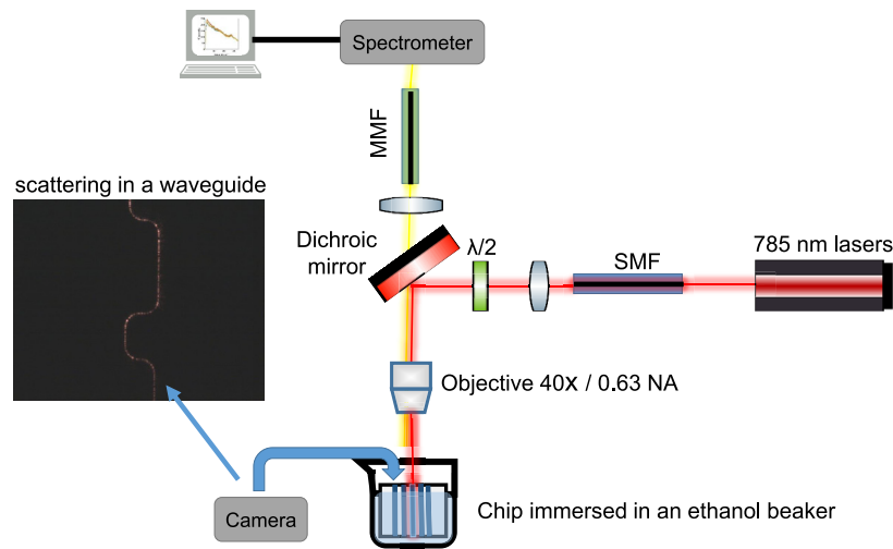
Fig. 3. The schematic of an optical setup used for Raman measurements. The left inset shows the light scattering of a waveguide imaged by the side camera. SMF = single mode fiber and MMF = multi-mode fiber.
