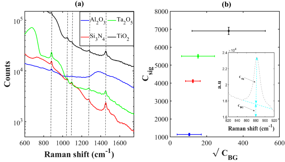
Fig. 6. a) The Raman spectra measured from an ethanol clad waveguides of Al_2O_3 , Si_3N_4 , Ta_2O_5 and TiO_2 . The dotted lines represent the 880, 1054, 1098, 1275 and 1456 cm^{-1} Raman modes of ethanol. b) The signal strength C_{sig} and background noise \sqrt{C_{BG}} measured for 880 cm^{-1} Raman mode of ethanol. The inset shows the C_{sig} and C_{BG} .
